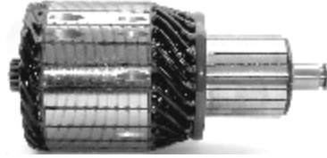
IM 3174 24V 6.0Kw Replacing: 2004014090, 874351 Servicing: 0001330001, 0001330003, 0001330004, 0001330007, 0001330008, 0001330011, 0001330012, ... Slots:23 Teeth:15 O.D.75,0 L.160,0
