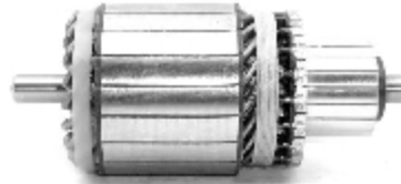
IM 536 12 V Replacing: 132027, 182049, 182175, 594148, NE407, NE410 Servicing: D9R105, D9R106, D9R116, D9R118, D9R119, D9R122, D9R126, ... Slots: 19 O.D.59,9 L. 137,0
