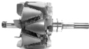
A/ 433 12 V 100 Amps Replacing: 233768 Servicing: LR1100-502E, LR1100-502F Teeth: 8 O.D. 107,5 L. 200,0
