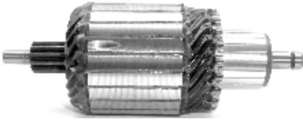
IM 3130 12 V 1.8 KW Replacing: 1004011211, 234166 Servicing: 0001110132, F000AL0108 Slots:23 Teeth:11 O.D.59,0 L. 160,0
