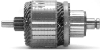
IM 3168 12 V 0.9 Kw Replacing: 020911311, 1004011214 Servicing: 0001120400, 0001120401, 0001120402, 0001120403, 0001120404, 0001120405, 0001120406, ... Slots:28 Teeth:11 O.D.52,0 L.107,5
