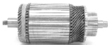
IM 305 24 V Replacing: 10626 Slots:41 O.D. 75,0 L. 193,0
