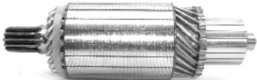
IM 3123 12 V Replacing: 23310-Z9004 Servicing: 03575020010, 23300-Z5519X Slots:21 Teeth:12 O.D.65,0 L.206,5
