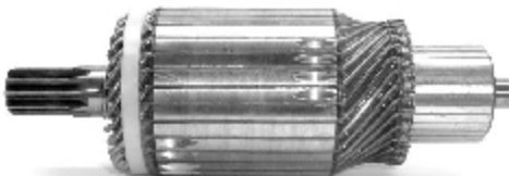
IM 3034/24 24 V Servicing: M4T95071 Slots: 33 Teeth: 10 O.D. 65,0 L. 196,5
