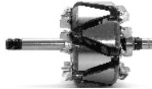
A/ 1192 12 V 200 AMPS. Servicing: 0124625063 O.D. 111,3 L. 194,0
