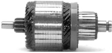
IM 3166 12 V 1.2 Kw Replacing: 06B911311, 1004011210, 330084 Servicing: 0001107402, 0001107407, 0001107409, 0001107410, 0001107417, 0001107421, 0001107427, ... Slots:28 Teeth:11 O.D.52,0 L.114,0
