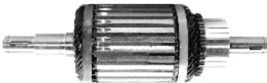
IM 332 24 V 800 W - Electric Pumps Slots:29 O.D. 73,0 L. 238,0
