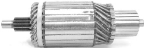
IM 3039 12 V Replacing: 139352, F4TZ11005A Servicing: F4TZ11002A, M8T50071, M8T50171 Slots:23 Teeth:13 O.D.53,6 L. 170,0
