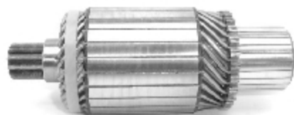
IM 3035 12 V Replacing: 137092, 2130-11001, 23310-54A00, 23310-J5501 Servicing: S13-41, S13-41A, S13-45B Slots: 25 Teeth: 11 O.D. 60,0 L. 165,0
