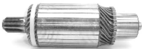
IM 3025 24 V Replacing: 136190, 2210-41001, 23310-99118 Servicing: S210-100, S210-98D, S210-98E Slots: 27 Teeth: 11 O.D. 65,0 L. 204,0
