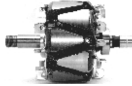
A/ 1191 24 V 80 AMPS. Replacing: 235054, F00M131616, F00M131645 Servicing: 0124555001, 0124555002, 0124555003, 0124555004, 0124555006, 0124555007, 0124555011, ... O.D. 103,2 L. 162,0
