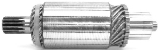
IM 3118 24 V Replacing: 132005901X0, 136518 Servicing: 03506020016, 03506020020, 03506020037, 03506020040, 03506020050, 03506020080, 03516020013, ... Slots:21 Teeth:14 O.D.65,0 L.215,0
