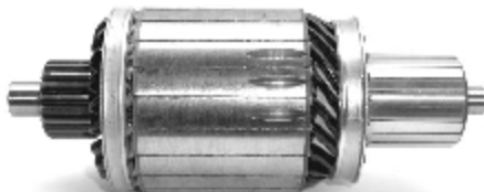
IM 3147 12 V 3.9 Kw Replacing: 10516266 Servicing: 19011506, 19011508, 19011514, 19011515, 19011516, 19011517, 19011518, ... Slots: 21 Teeth: 20 O.D. 68,0 L. 196,0
