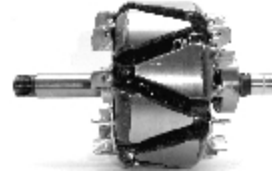
A/ 1194 24 V 90 AMPS. Replacing: 1124035530, 1124035543, 234523, 81261020039 Servicing: 0123525501 O.D. 111,3 L. 177,0
