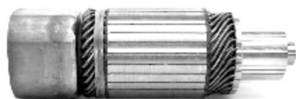
IM 105 24 V Replacing: 131311, 2004005023, 2004005024, 2004005028, 353381, 5000816636, 5000821022, ... Servicing: 0001417001, 0001417002, 0001417005, 0001417006, 0001417007, 0001417008, 0001417012, ... Slots: 29 O.D.83,0 L.256,0
