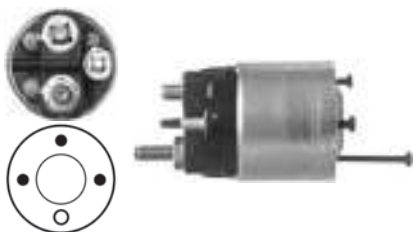
236859 Solenoid Replacing: 594461 Servicing: D6RAD183, D6RADP359 12 V, B+ M8, Kl. 50 M6, ID/ cover 23.95, OD 51.40, OD/ cover 47.20, Total length 88.65, Height/ B+ 8.75, Width/ kl. 50 10.40, Coil bolt M8, Coil bolt 2 16.80, No./ terminals 3
