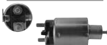
330427 Solenoid Servicing: tm000a38001 12 V, B+ M8, Kl. 50 Plug, OD 49.76, Total length 125.00, Height/ B+ 15.00, Coil bolt M8, Coil bolt 2 13.00, No./ terminals 3
