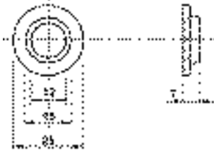
610188 Bushing
