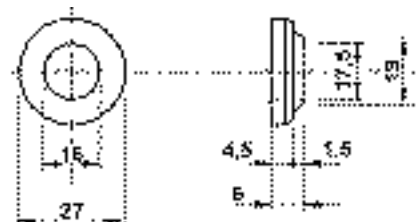
610057 Rubber Bushing
