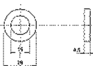
610056 Rubber Bushing
