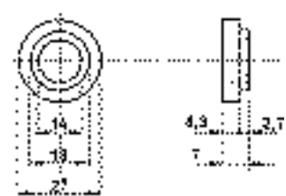
610058 Rubber Bushing
