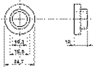
610060 Steel bush
