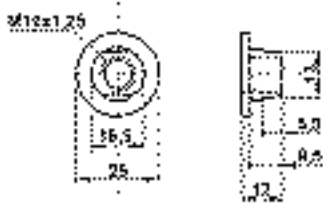
610052 Bushing
