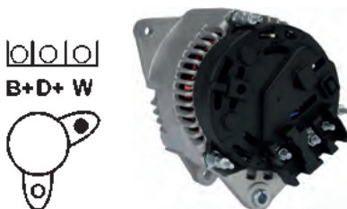
112718 Alternator 14 V, 100 Amp Replacing: AAK5326, 11.203.042 Servicing: Ford, New Holland Terminal W, Grooves 6, Total length 189.00, Pulley SP, Fan IF A: 32.00 B: 14.00 C: 83.80 mm
