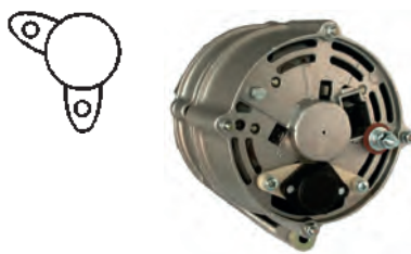
112736 Alternator 14 V, 65 Amp Replacing: AAK1378, 11.201.570 Servicing: Deutz-Fahr, Fahr, Iveco Terminal W, Grooves 1, Total length 166.00, Pulley P, Fan EF A: 76.50 B: 56.10 mm
