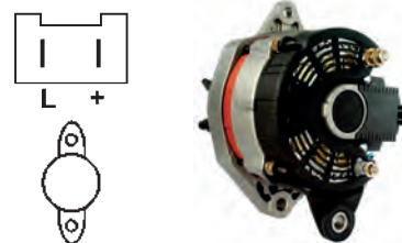
112744 Alternator 14 V, 60 Amp Replacing: AAK3591, 11.201.532 Servicing: Renault, Volvo Grooves 5, Total length 162.50, Pulley SP, Fan EF A: 45.00 B: 27.00 C: 66.00 mm
