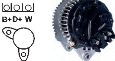
112698 Alternator 14 V, 100 Amp Replacing: AAK5580, 11.203.433 Servicing: Ford Terminal W, Grooves 6, Total length 178.00, Pulley SP, Fan IF A: 33.00 B: 14.10 C: 83.30 mm
