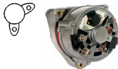
112747 Alternator 28 V, 55 Amp Replacing: AAK5734, AAK3318, 11.203.655, 11.201.903 Servicing: Deutz-Fahr, Ford, Iveco, KHD Terminal W, Total length 177.00, Pulley w/o, Fan EF B: 56.00 mm
