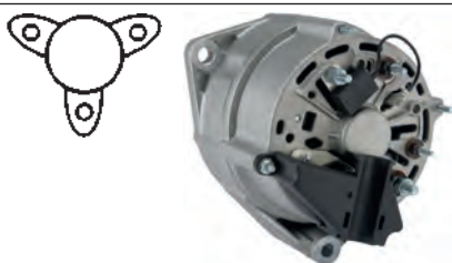
112561 Alternator 28 V, 80 Amp Replacing: AAN3119, AAN3111, 11.209.442, 11.209.421 Servicing: Mercedes-Benz Terminal W, Total length 188.00, Pulley w/o, Fan EF B: 80.00 mm
