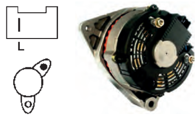
112754 Alternator 14 V, 70 Amp Replacing: AAK4542, 11.201.679 Servicing: Citroen, Peugeot Grooves 1, Total length 172.50, Pulley P, Fan EF A: 95.00 B: 56.00 mm
