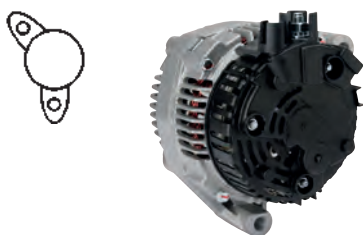
112688 Alternator 14 V, 95 Amp Replacing: AAK5186, 11.201.963 Servicing: Alfa Romeo, Citroen, Fiat, Lancia, Peugeot Grooves 6, Total length 175.00, Pulley SP, Fan IF A: 92.50 B: 55.80 mm
