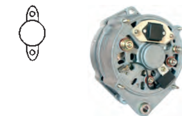
112757 Alternator 28 V, 55 Amp Replacing: AAN3115, 11.209.435 Servicing: Scania, Volvo Terminal W, Total length 185.00, Pulley w/o, Fan EF Bosch 0 120 469 963 = Insulated, HC-CARGO 112757 is not insulated. B: 27.50 C: 68.00 mm
