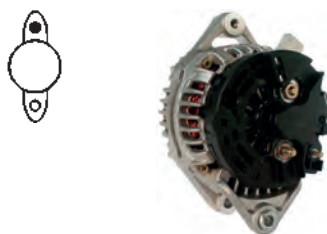
112720 Alternator 14 V, 100 Amp Replacing: AAK5722, 11.209.439 Servicing: Opel, Vauxhall Grooves 1, Total length 173.00, Pulley P, Fan IF A: 53.50 B: 33.40 C: 57.00 mm
