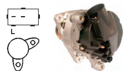
112654 Alternator 14 V, 90 Amp Manufacturer: Marelli Replacing: AAK5597, 11.209.429 Servicing: Ford Total length 213.00, Pulley w/o, Fan IF B: 17.25 C: 62.60 mm
