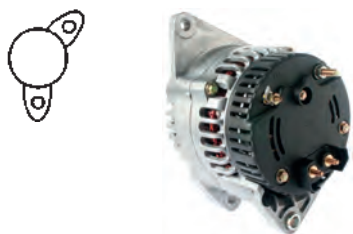
112679 Alternator 14 V, 110 Amp Replacing: AAN5139, AAK5521, 11.203.227, 11.203.129 Servicing: Renault, Volvo Terminal W, Grooves 6, Total length 190.00, Pulley SP, Fan IF A: 46.50 B: 27.70 C: 66.30 mm
