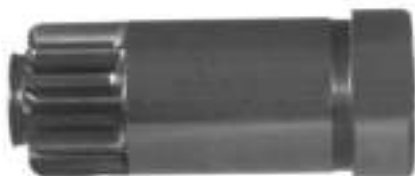
136679 Gear Wheel ID 12.70, OD 25.15, Height 65.70, No./ teeth 9
